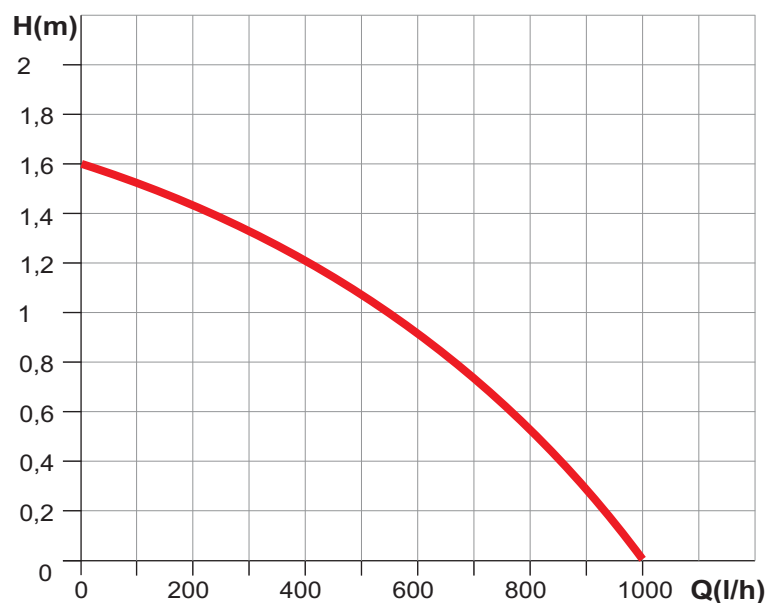
Dijagram protoka pumpi AQUA JET 1000
